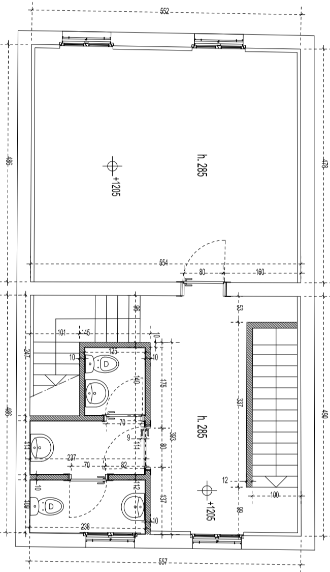
PIANO TERRA
